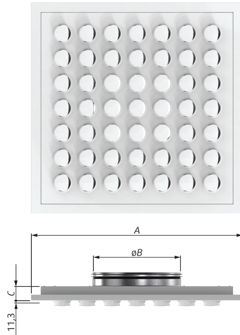
Fig. 1: CAP-F dimensions
